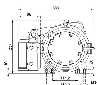
Air Clutch
